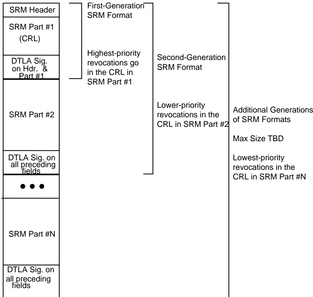
Figure 19 SRM Extensibility
